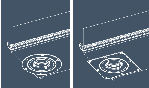
6/8" ROUND/ SQUARE GRILLE ADAPTER
