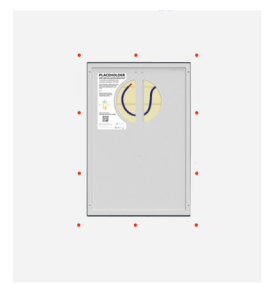
INSTALL WALLBOARD
