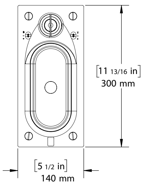
Outer Dimension
